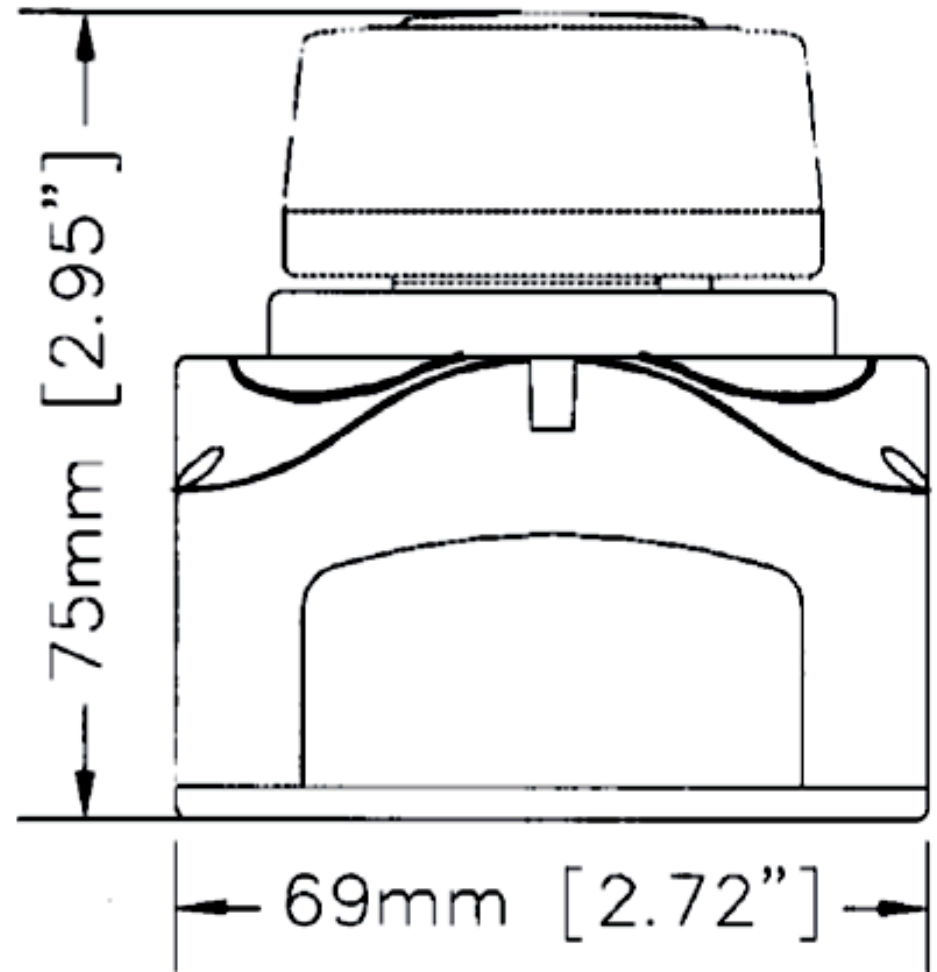
SIDE VIEW
