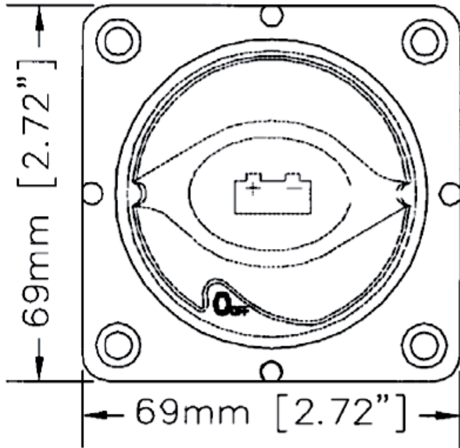
FRONT VIEW
