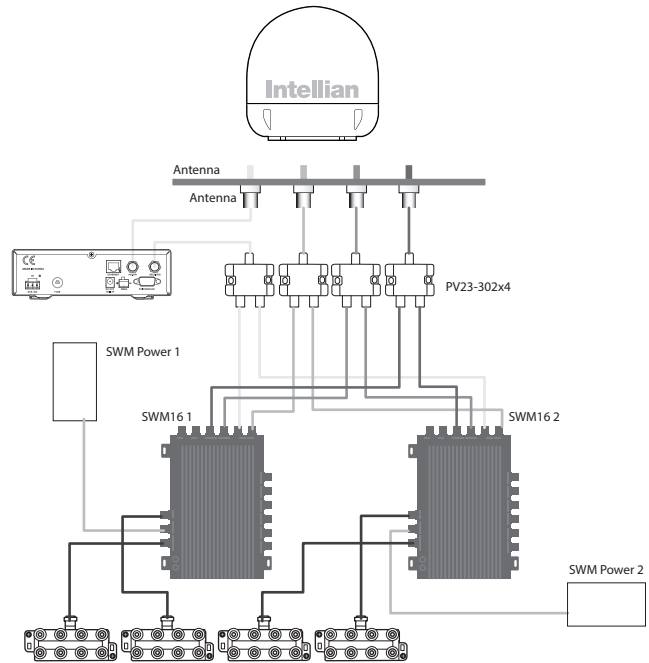
Figure 16 : 32 Receivers Connection
