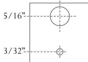
Mounting Template
