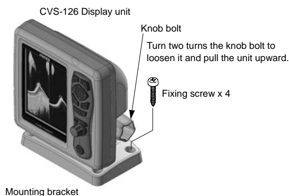
Fig. 5.2 Desk-top Installation
