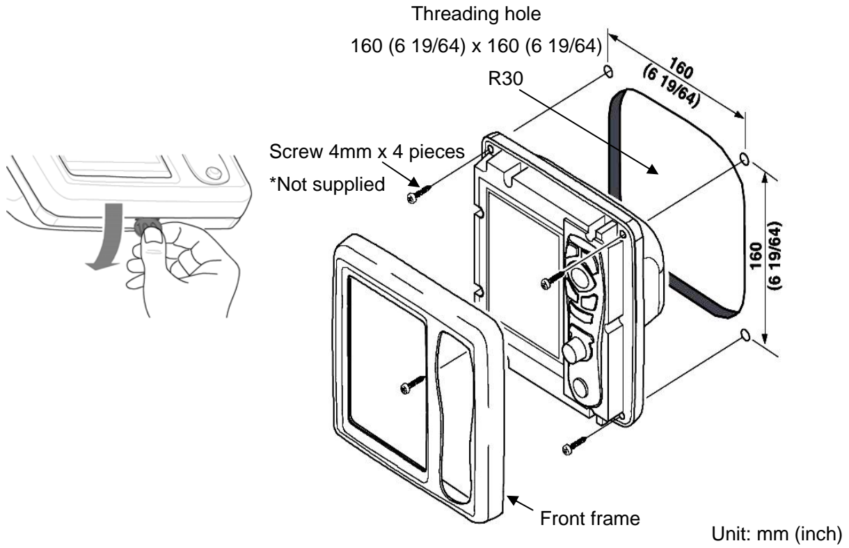
Figure 5.3 Flush-mount Installation
