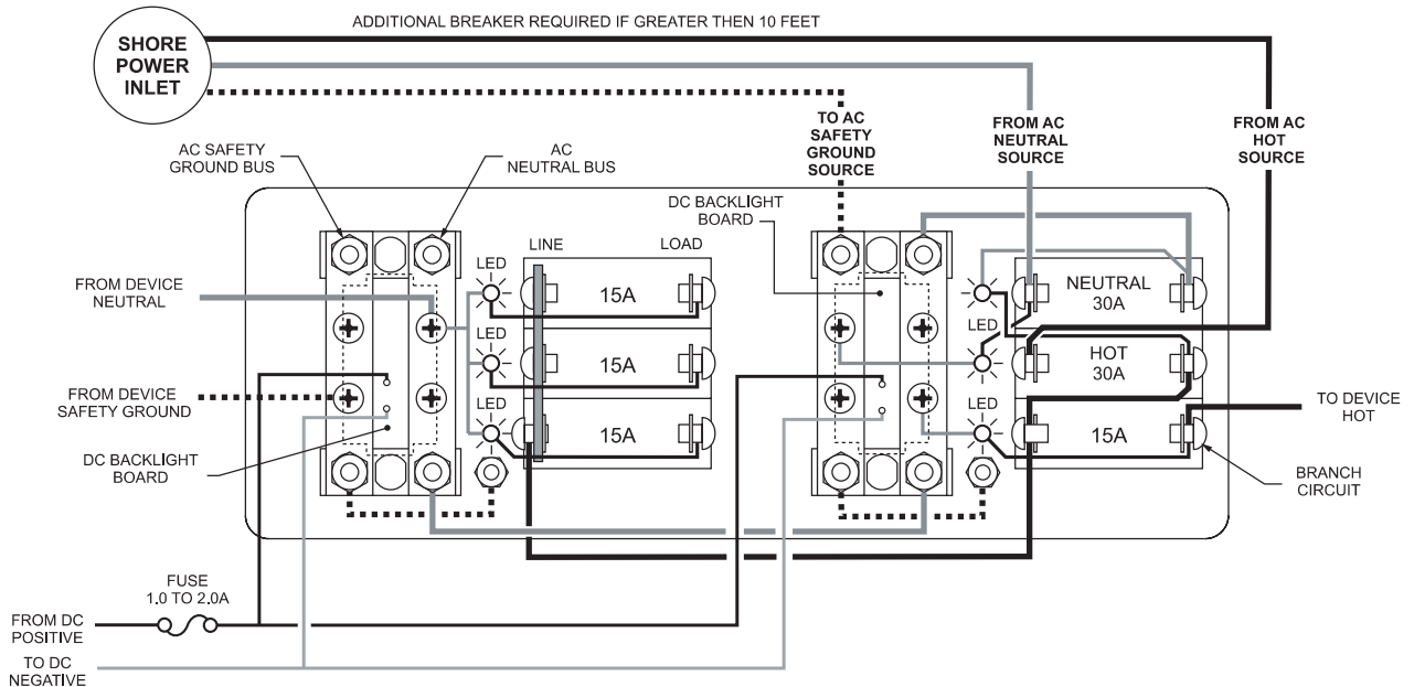
Wiring Diagram AC Power Distribution Panel (PN 8099 / PN 3099 shown for reference)
